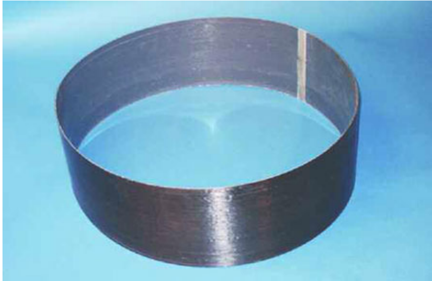
Figure 9 Carbon fiber plate lapped in a circular orientation Image from http://www.fortressstabilization.com/strap.php
